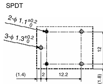
Mounting Holes (Bottom View) Tolerance: \pm 0.1 mm Unless specified
